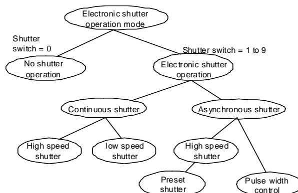
Fig. 5-1 Electronic shutter operation modes
