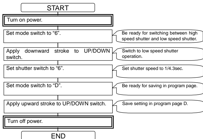
Fig. 6-3 Procedure 1 for use in continuous/low speed shutter operation (1/4.3 sec.)
