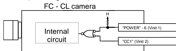
Fig. 4-2 Internal connection of Vinit signals
