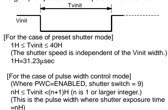
Fig. 4-3 Recommended Vinit signal timing waveform
