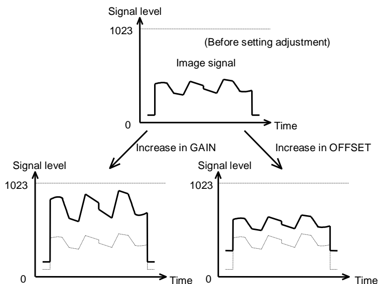
Fig. 5-2 Conceptual diagram of gain and offset levels
