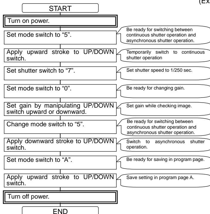
Fig. 6-2 Example of procedure for gain setting for random shutter
