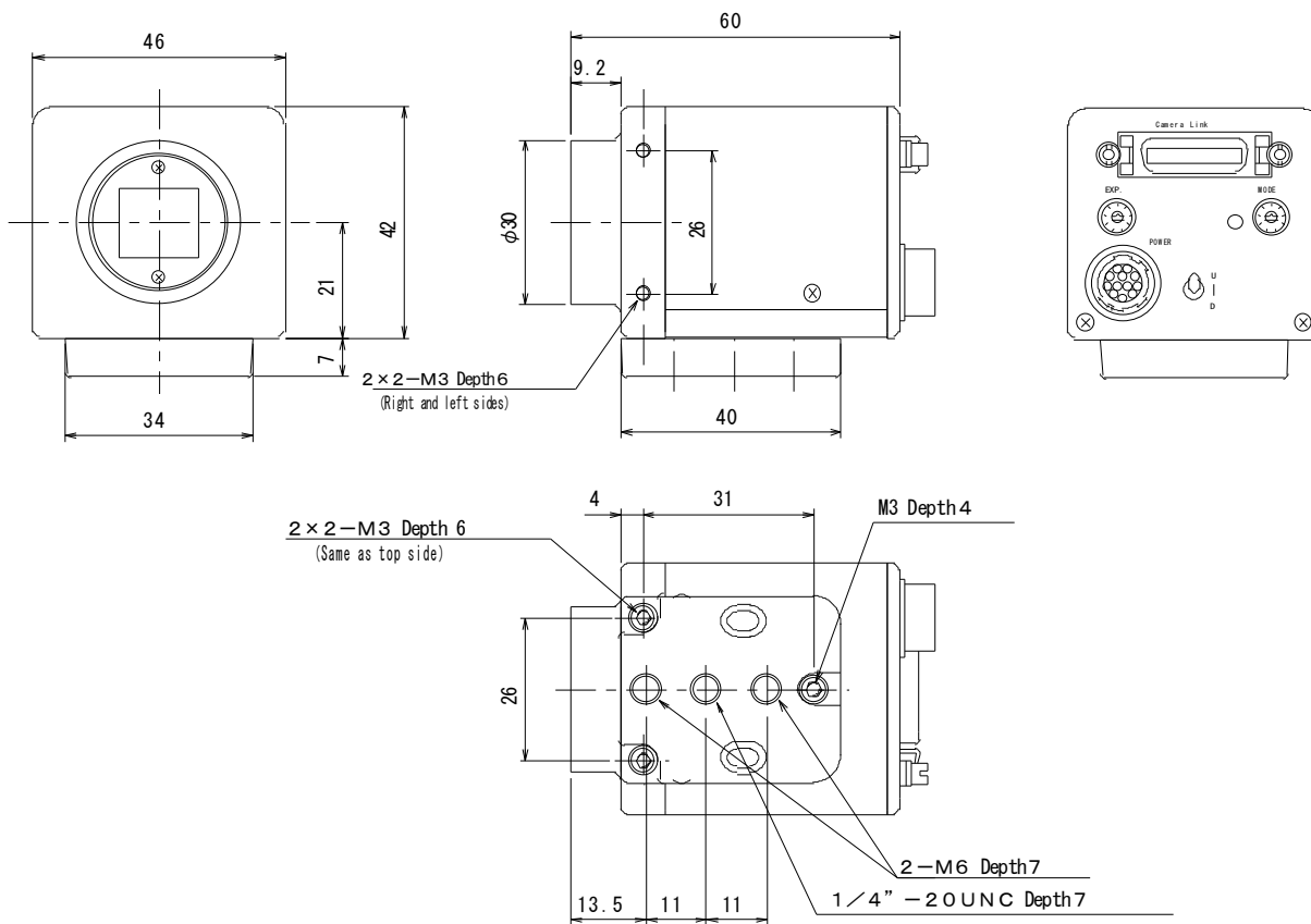
Fig.11-1 FC1600FCL external views
